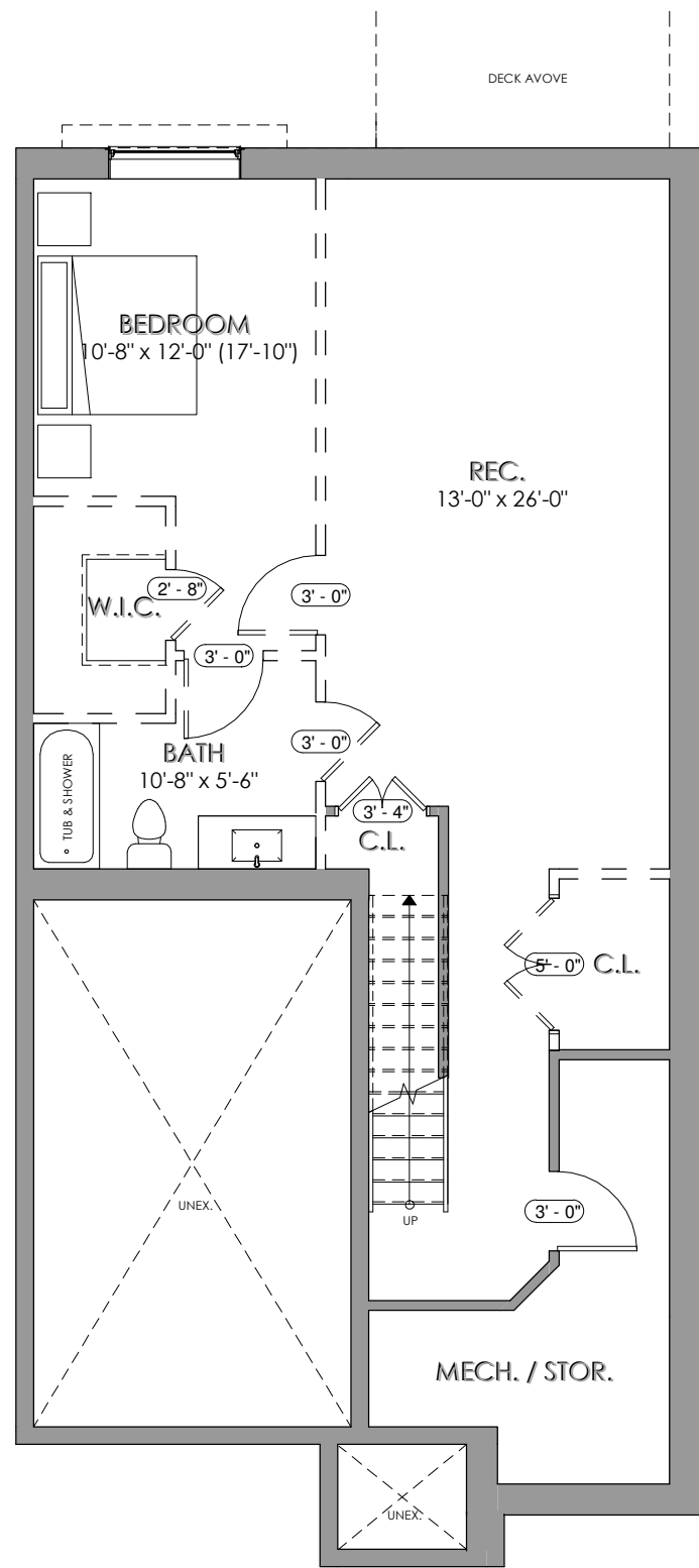
LOWER FLOOR 842.19 SQ.FT (OPTIONAL)
